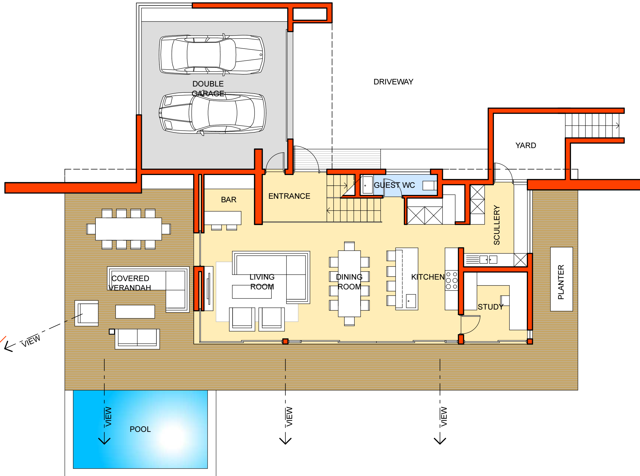
UNIT TYPE H LEVEL 0 - FLOOR PLAN SCALE 1:100
